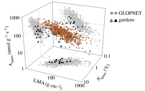
Figure 5. The three-dimensional relationship between LMA, N, A_{\max} traits of the leaf economic spectrum. Orange dots and blue triangles represent the three-dimensionality of the data for GLOPNET and FTBG data, respectively. Grey dots and black triangles represent the two-dimensional relationships of the LES traits.
